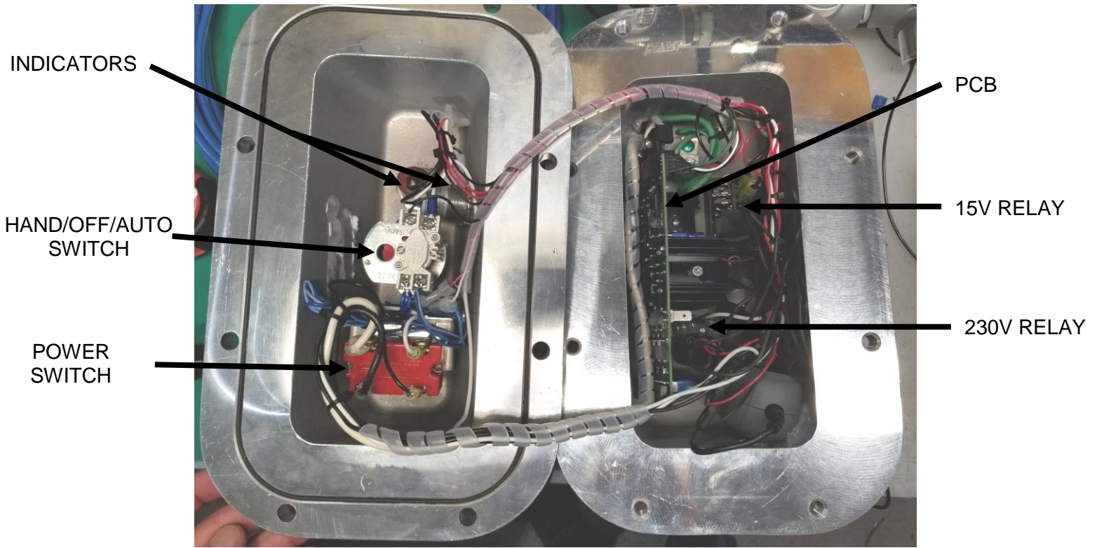
Figure 5-2: Internal Components (New)
