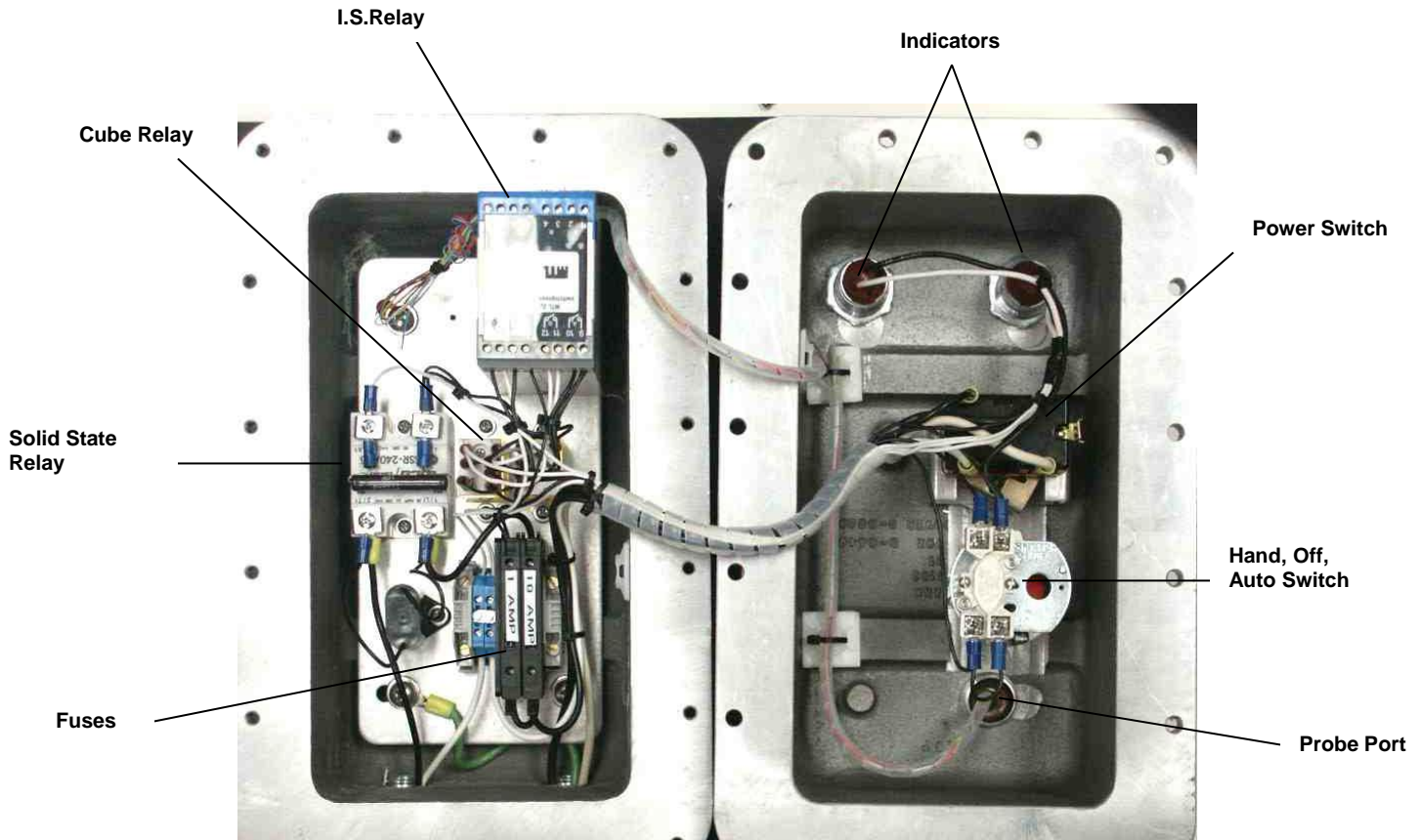
Figure 5-1: Internal Components (old)
