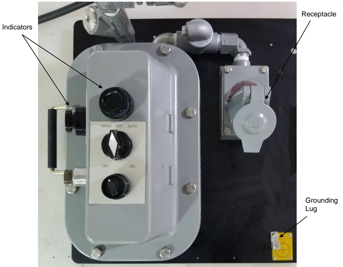
Figure 1-4: The Water Table Depression Pump Control Module (New version)
