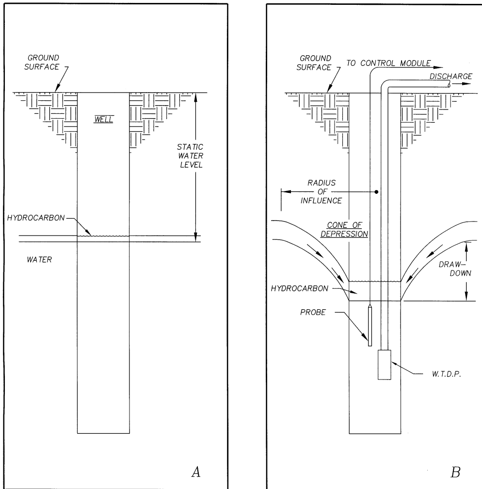
Figure 1-1: A hydrocarbon recovery well before (A) and after (B) installation of a Water Table Depression Pump
