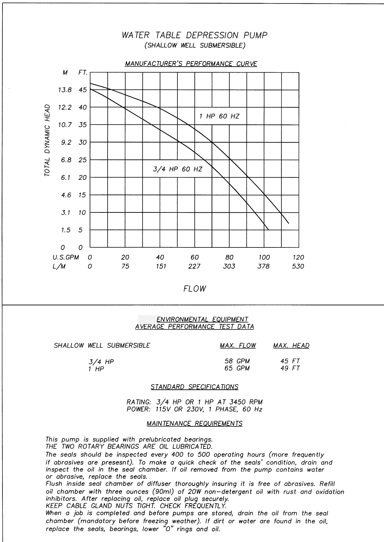
Figure 7-1: WTDP Performance Curves
