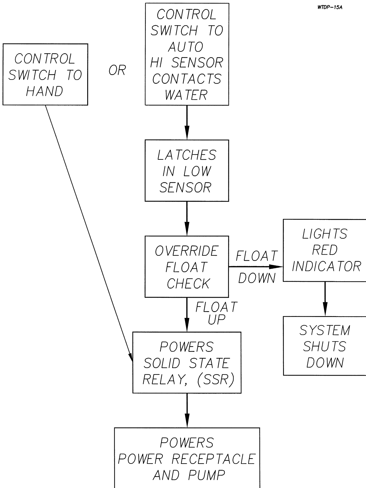
Figure 1-2: Logic Diagram for Water Table Depression Pump
