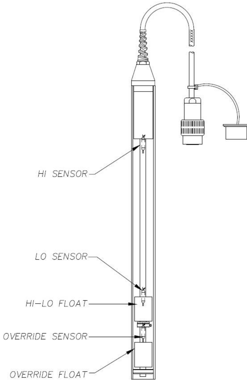
Figure 1-5: Water Table Depression Pump Density Probe
