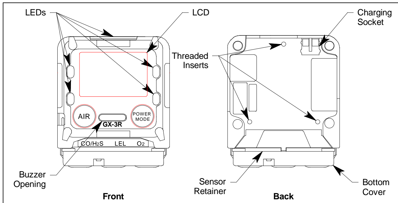
Figure 1: Component Location
