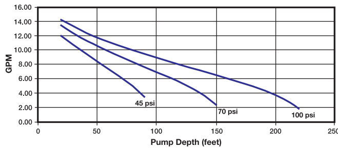
36" Dual Loading Fixed Intake (3/4" ID Fluid Discharge Hose)
