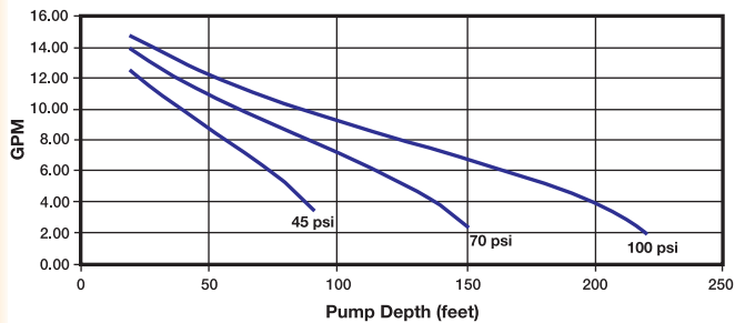
60" Dual Loading Fixed Intake (3/4" ID Fluid Discharge Hose)
