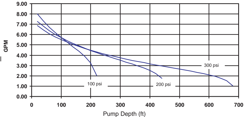
Geotech 3.5 Reclaimer
