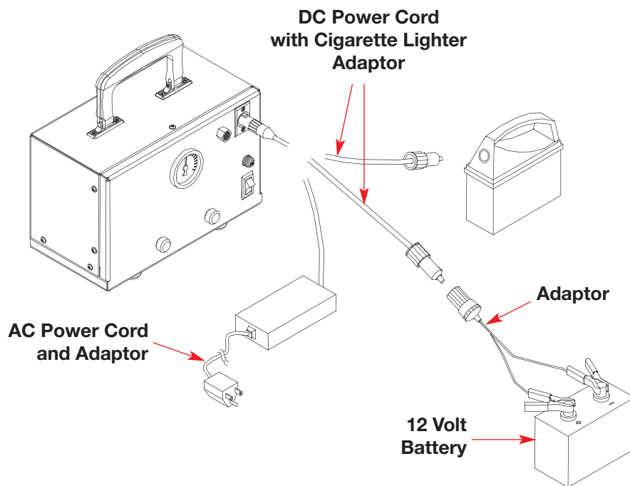
Figure 1 Installation Diagram
