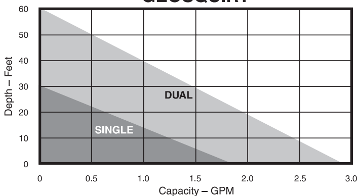
PUMPING CURVES FOR GEOSQUIRT
