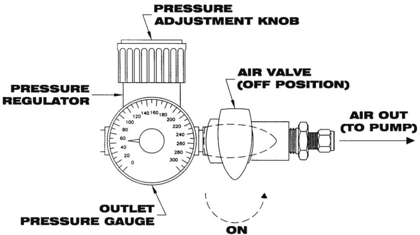
Figure 3-1 – Air Supply
