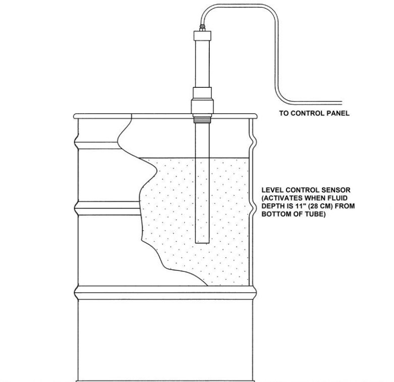
Figure 1-5 – Example of the Tankfull Shut-off Sensor (recovery tank not supplied)
