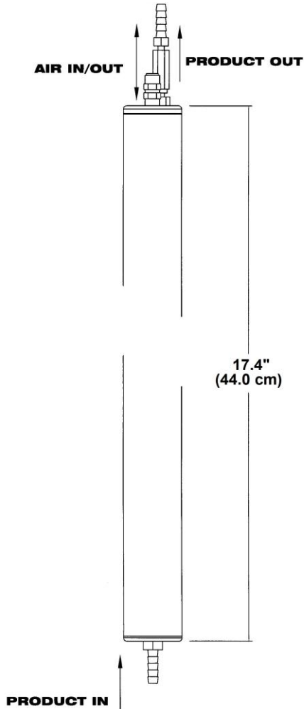
Figure 1-1 – PRS Pump
