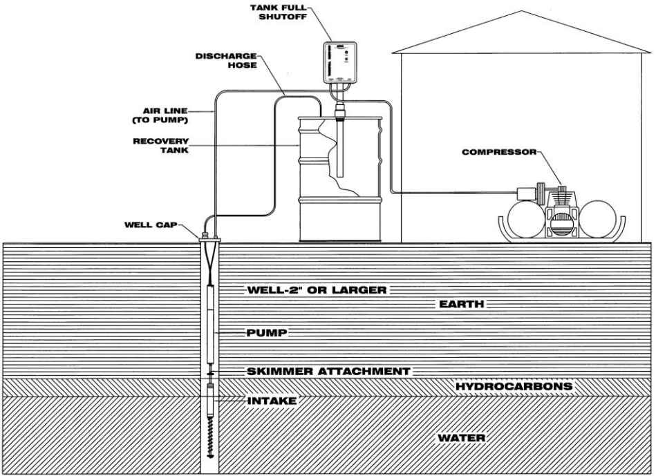
Figure 7-2 – Typical Site Installation with optional Tankfull Shut-off and Manual Restart
