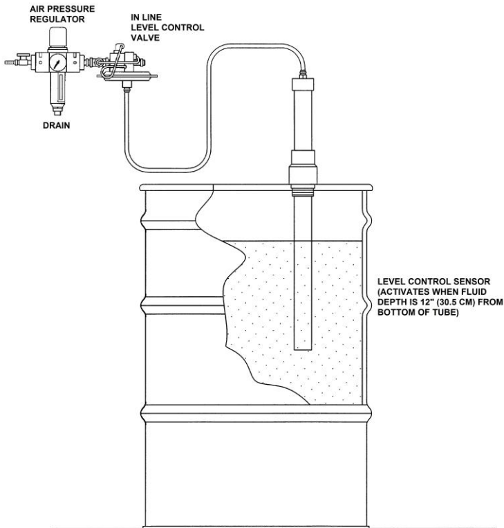
Figure 1-4 – Example of the Tankfull Shut-off Sensor (recovery tank not supplied)
