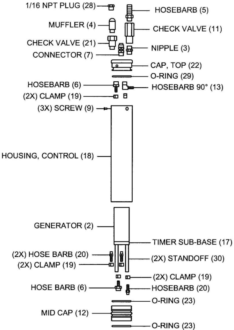
Figure 8-1 – Upper Half of SpOiler Pump Assembly
