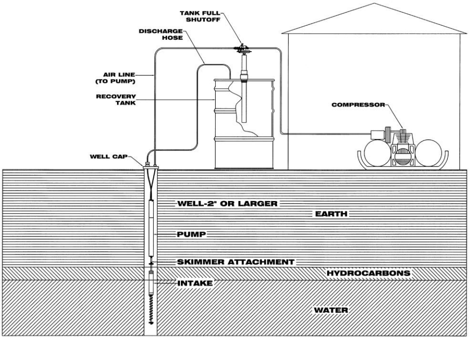
Figure 7-1 – Typical Site Installation with optional Tankfull Shut-off
