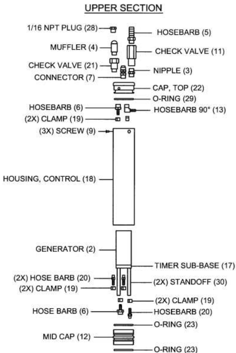
Figure 8-1: Upper Half of SpO 2 Pump Assembly
