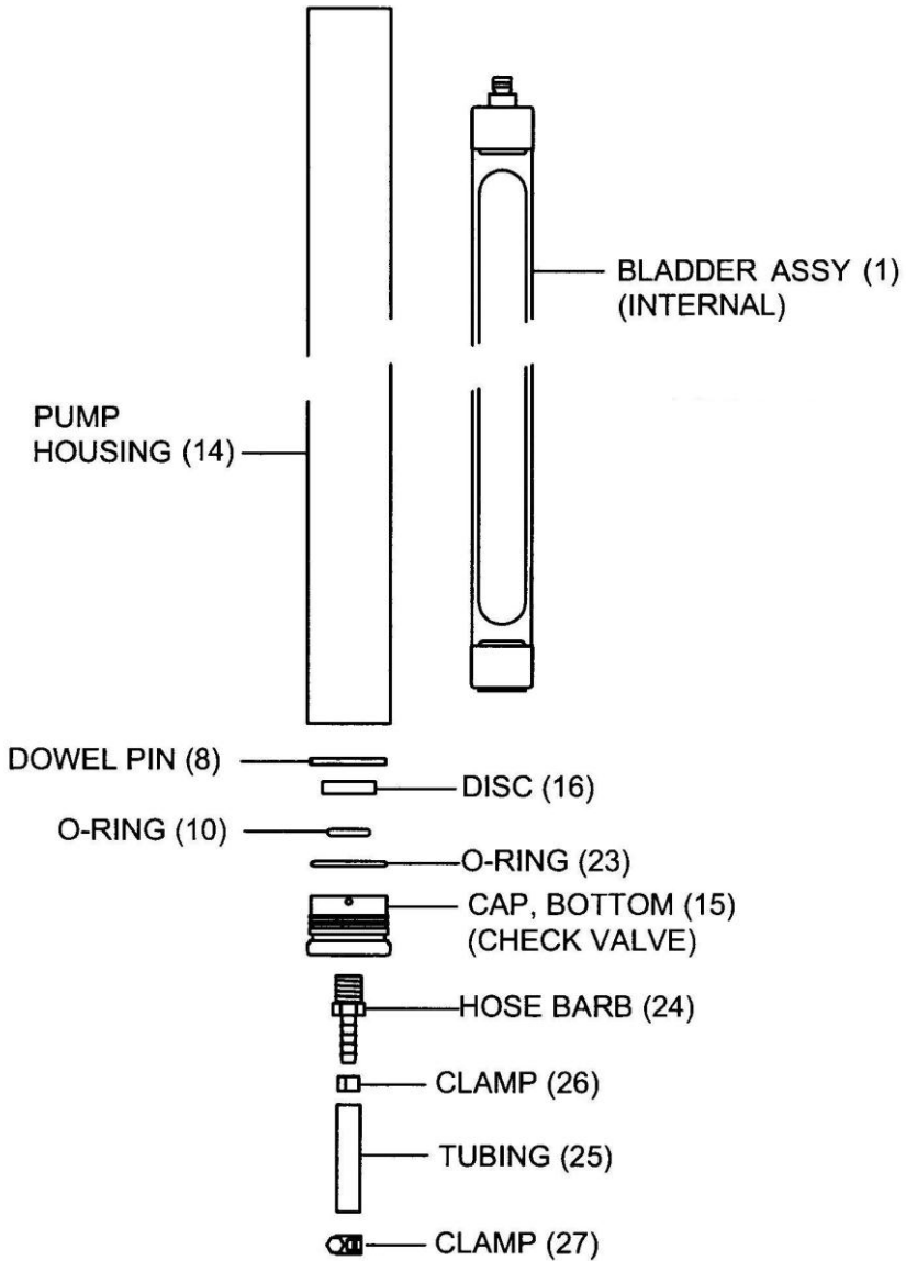
Figure 8-2 – Lower Half of SpOILer Pump Assembly
