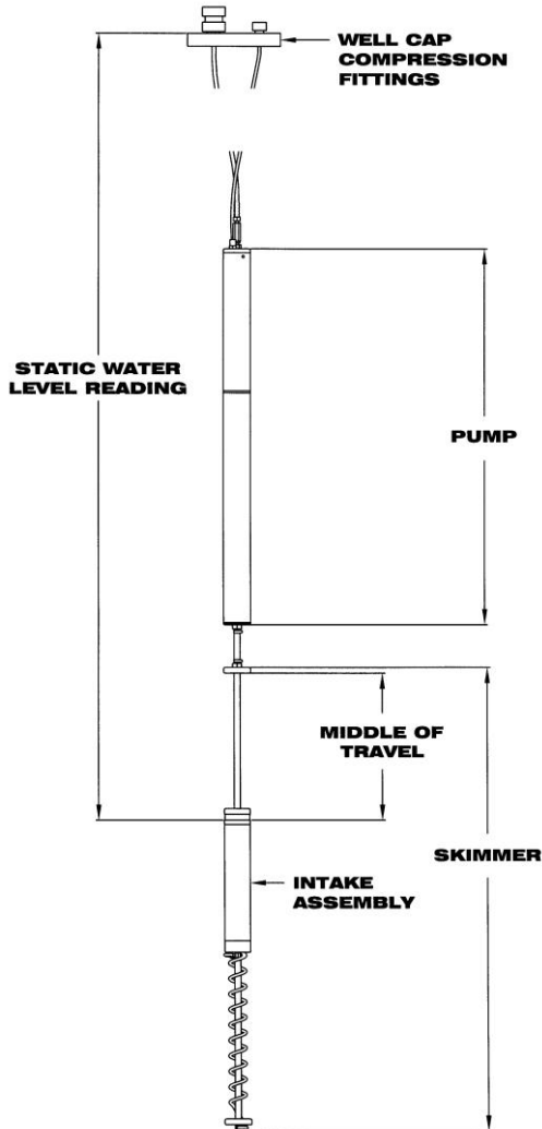
Figure 2-1 – Pump and Skimmer Assembly with Well Cap
