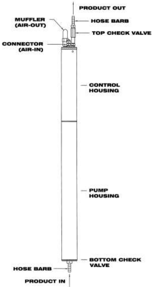
Figure 1-1: Pump
