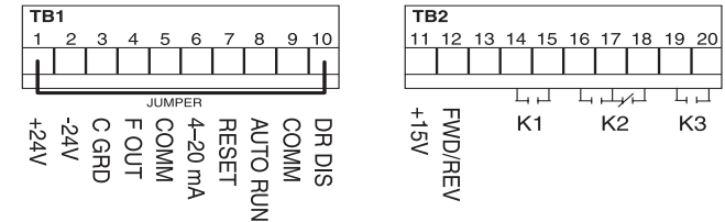
Figure 11: Diagram of input and output terminals located on top circuit board (behind cover)
