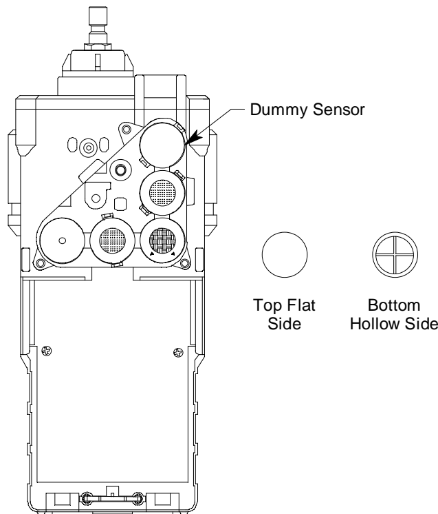
Figure 3: Dummy Sensor
