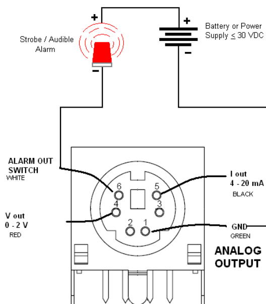
Figure 7-1. pDR-1500 External Alarm Driver
