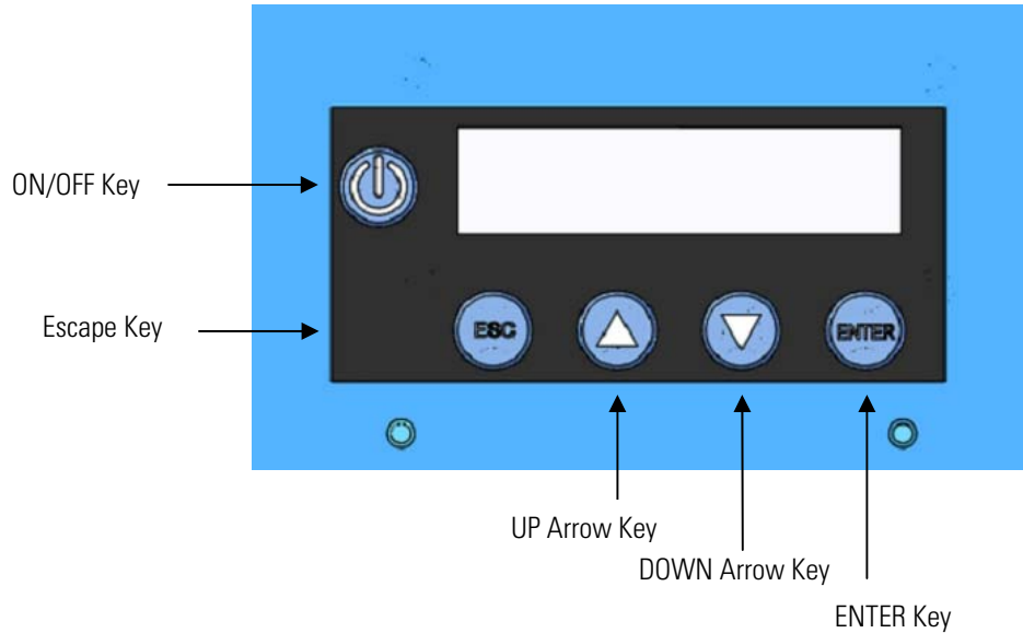
Figure 3–2. Keypad Functions
