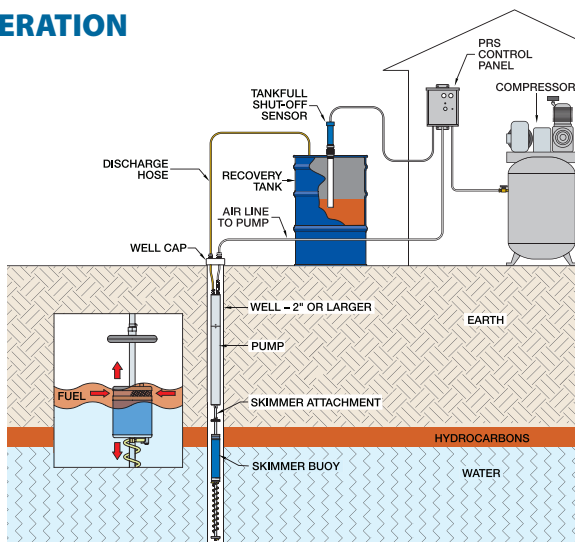
Typical PRS Installation with Tankfull Shut-Off Sensor
