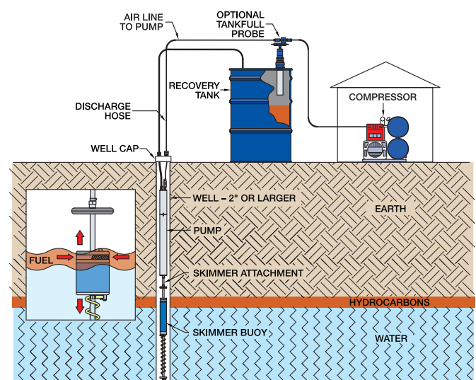
Typical SpOILer Installation
