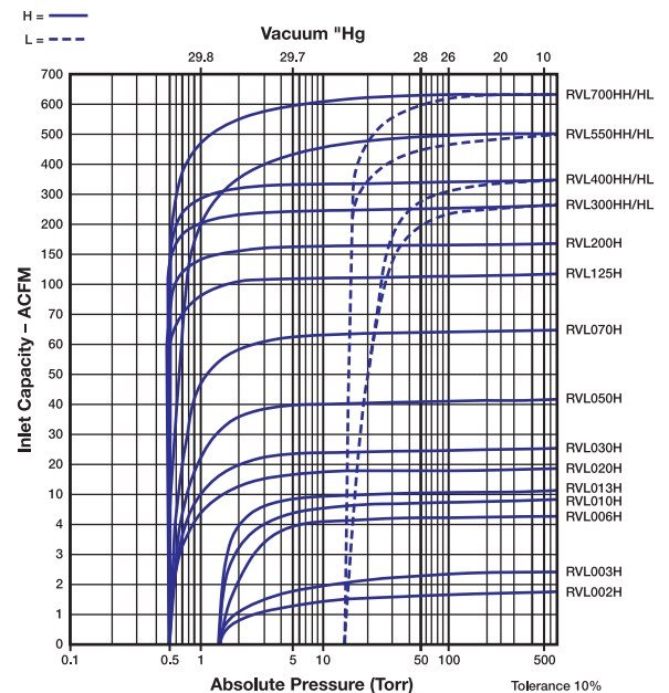
Performance Curves DuraVane Lubricated Rotary Vane Pumps
