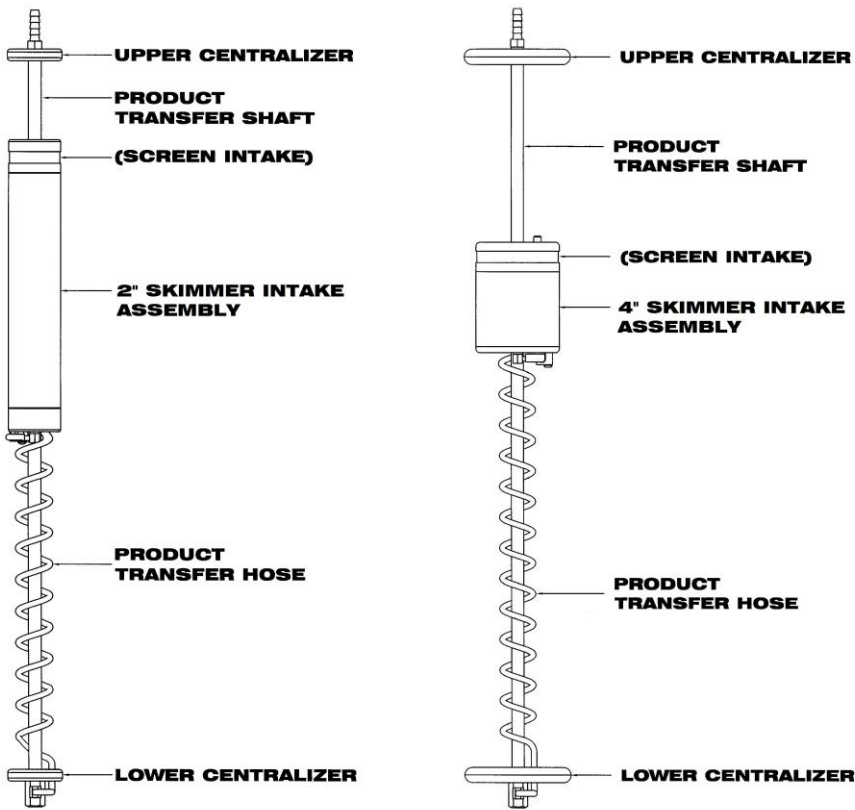
Figure 1-2: Standard 2" and 4" Skimmer Attachments
