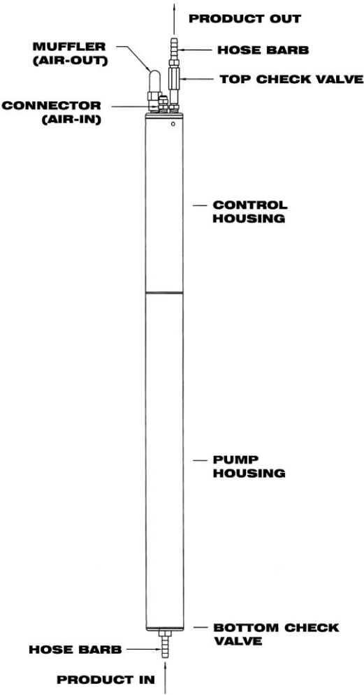
Figure 1-1: Pump
