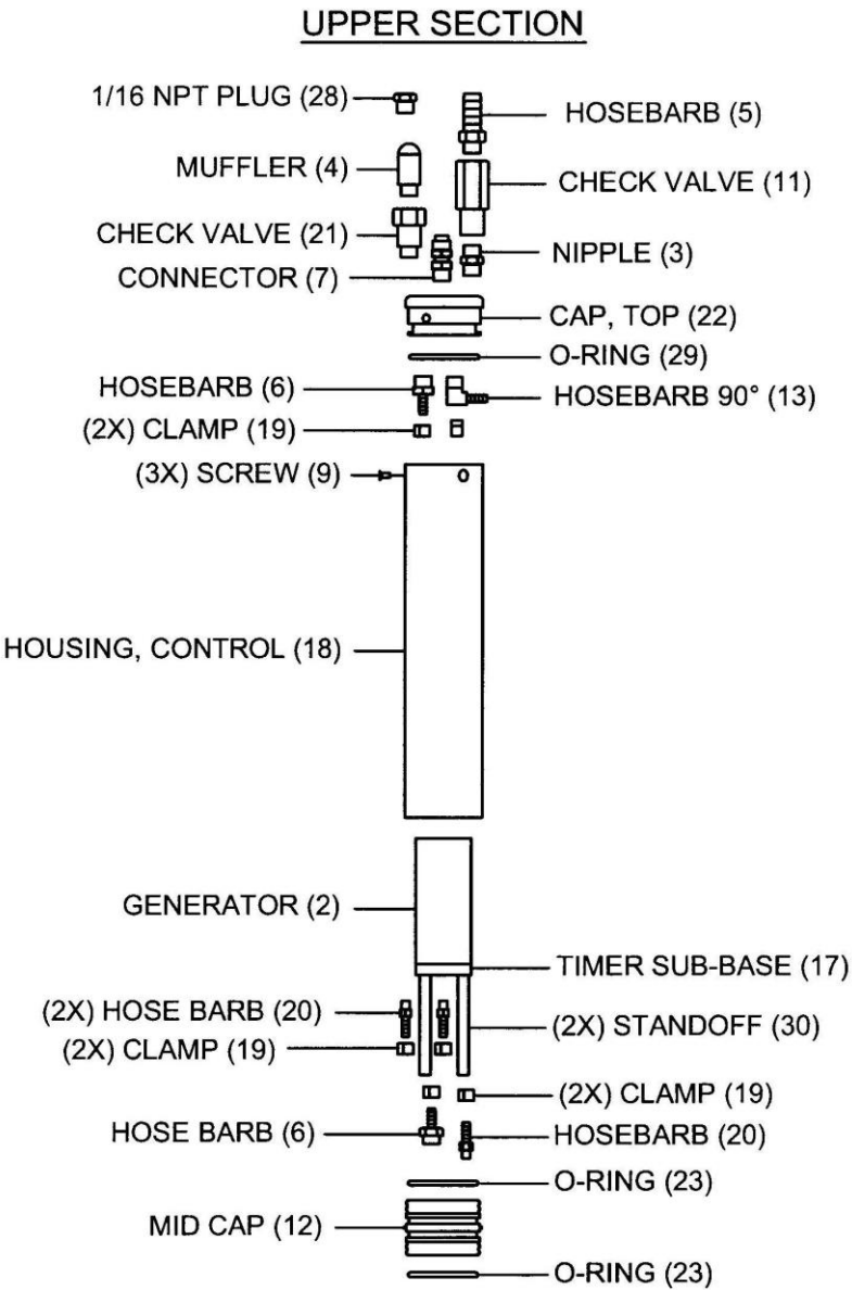
Figure 8-1: Upper Half of SpOiler Pump Assembly
